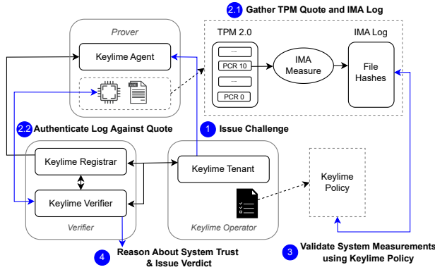
Fig. 1: Relationship between Keylime components, TPM 2.0, and Linux Integrity Measurement Architecture (IMA).
